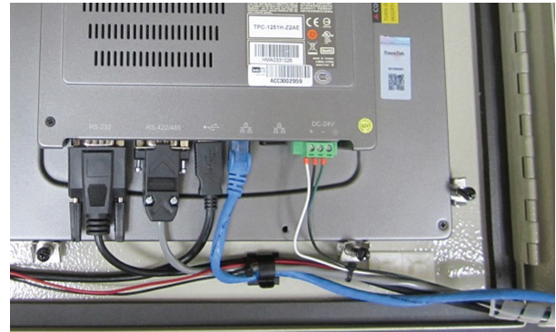
Ethernet connections to the TT-TS12 are made with a standard RJ-45 connector to either of two network ports on the rear side of the touch screen computer at the base
